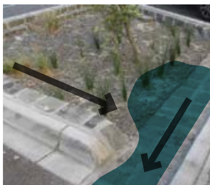
Surface of biofilter not flat, slope follows fall of road – poor distribution of flow
