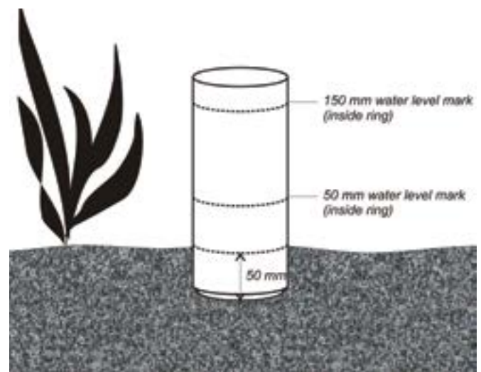
Figure 2. Diagram of single ring infiltrometer.
