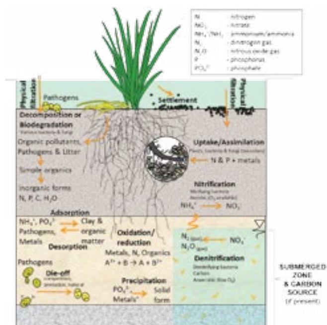
Figure 4. Key processes involved in pollutant attenuation, removal or transformation in stormwater biofilters
