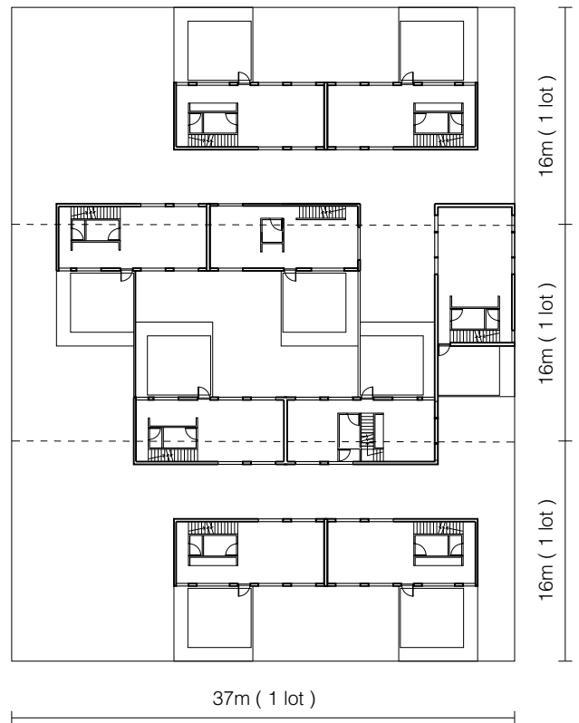
first floor plan 1 / 500
