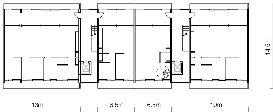
plan 1 / 500
