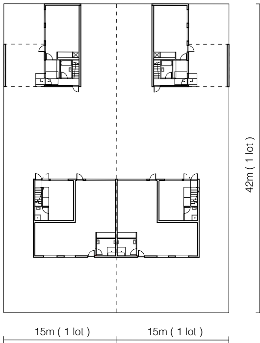
ground plan 1 / 500
