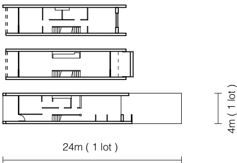
plan 1 / 500
