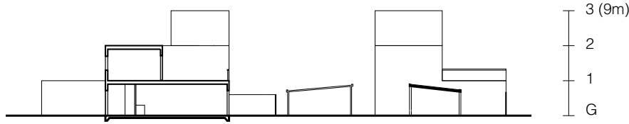
section 1 / 500
