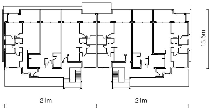
plan 1 / 500
