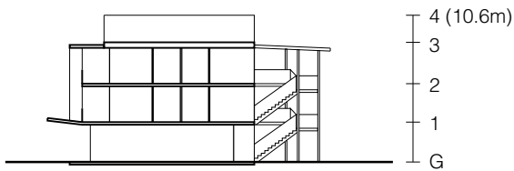
section 1 / 500
