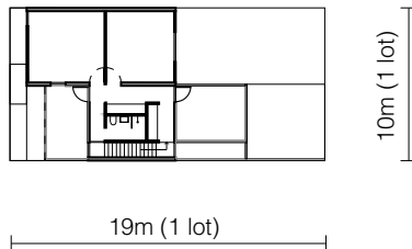
ground plan 1 / 500
