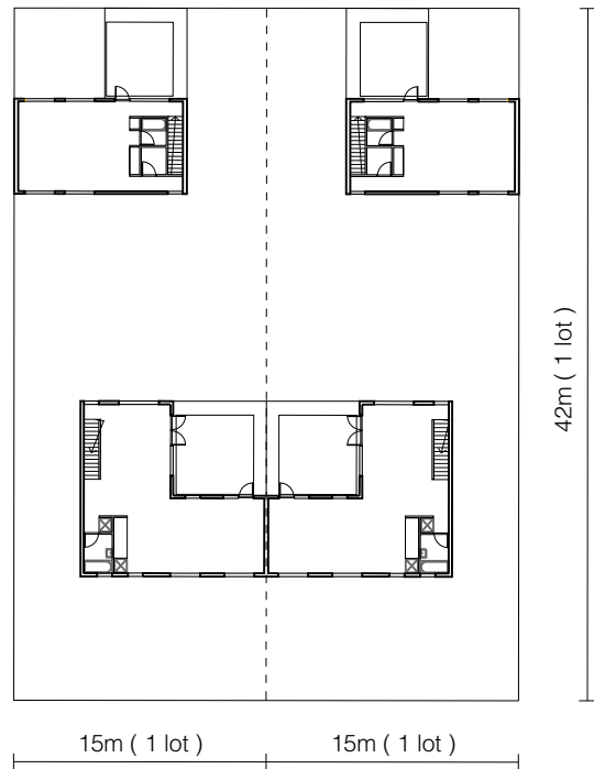
first floor plan 1 / 500
