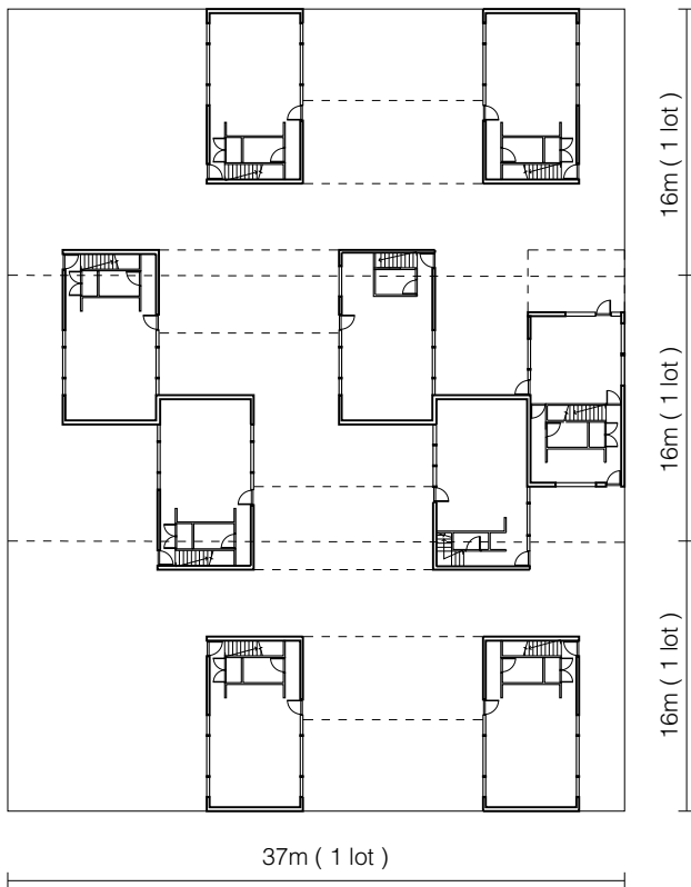
ground plan 1 / 500
