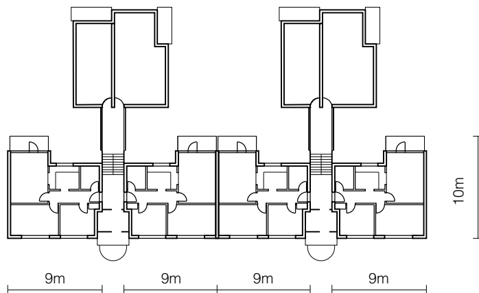
plan 1 / 500
