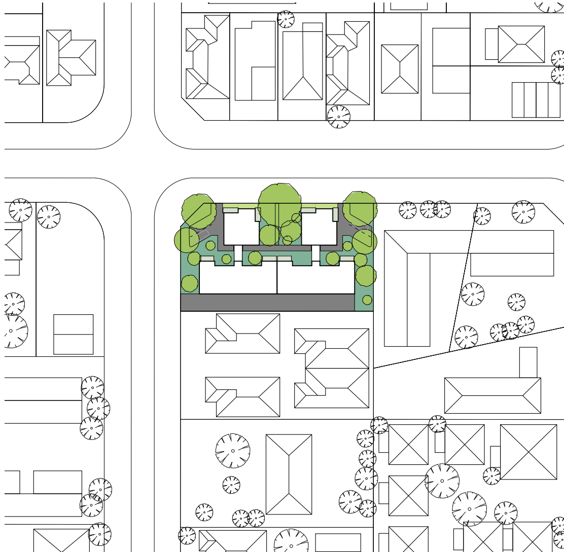
context plan 1/1000
