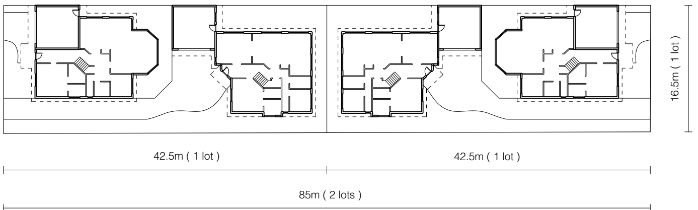
plan 1 / 500
