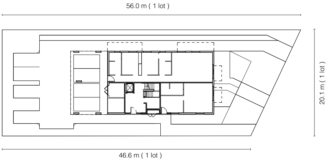
plan 1 / 500
