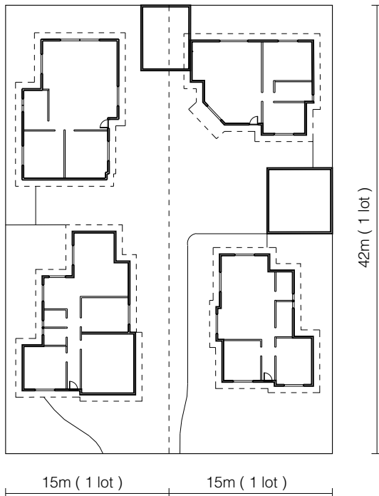
plan 1 / 500
