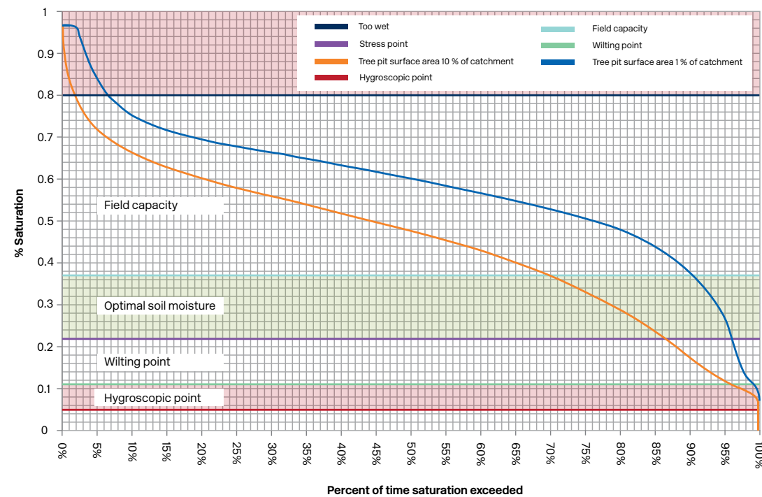
Figure 19 - Blacktown soil moisture curve showing tree pits with loamy sand, a high water use tree and no wicking zone will experience dry conditions (wilting point) less than 5% of the time
